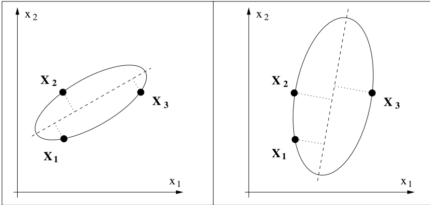
Fig. 3.6. Ellipses fitted through three points; (Left) Ellipse determined by PCA, showing first principal axis, determined by maximizing the variance; (Right) Ellipse determined manually with less variance along the first principal axis.
