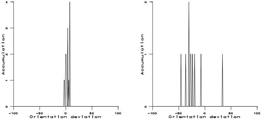
Fig. 2.55. Histograms of estimation errors for edge orientation; (Left) Diagram for operator version 5; (Right) Diagram for operator version 13.
