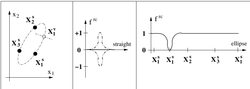
Fig. 3.38. (Left) Ellipse through three seed vectors and perpendicular straight line through a counter vector located on the ellipse; (Middle) Along the straight line the positive Gaussian course of proximity values is added with the negative Gaussian originating from the counter vector, resulting in 0; (Right) Along the ellipse the recognition values locally decrease at the position of the counter vector.
