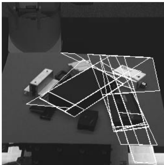
Fig. 2.22. Based on a saliency measure a subset of most conspicuous, approximate parallelogramms have been extracted.
