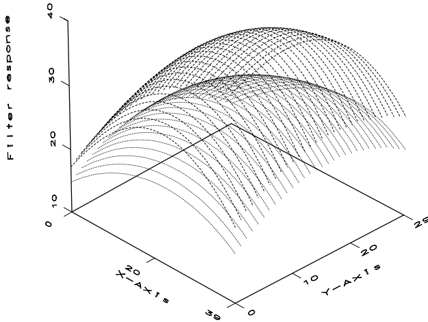
Fig. 3.18. The product combination of two orthogonal directed Gabor wavelet functions can be applied to the image patch of grasping situations. This filter responds specifically to certain relations between target object and grasping fingers. The overlay of the filter response patterns for two different grasping situations are shown. According to this, we can represent the finger-object relation by filter responses and avoid the difficult extraction of symbolic features.
