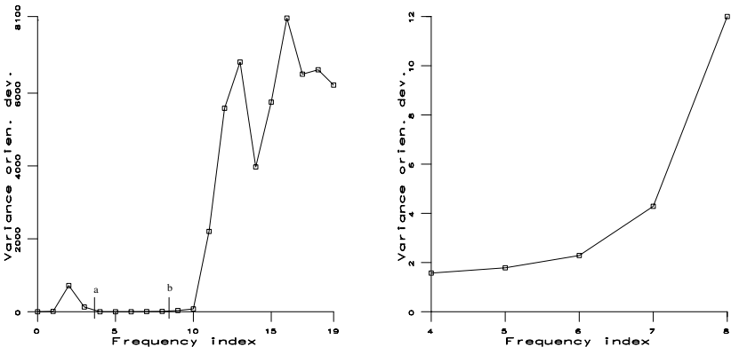
Fig. 2.52. (Left) Variance of estimation errors of edge orientation for 20 operators; (Right) Higher variance resolution of relevant section.
