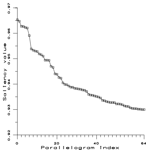
Fig. 2.23. Decreasing course of saliency values for the subset of extracted parallelograms in the image of Figure 2.22.
