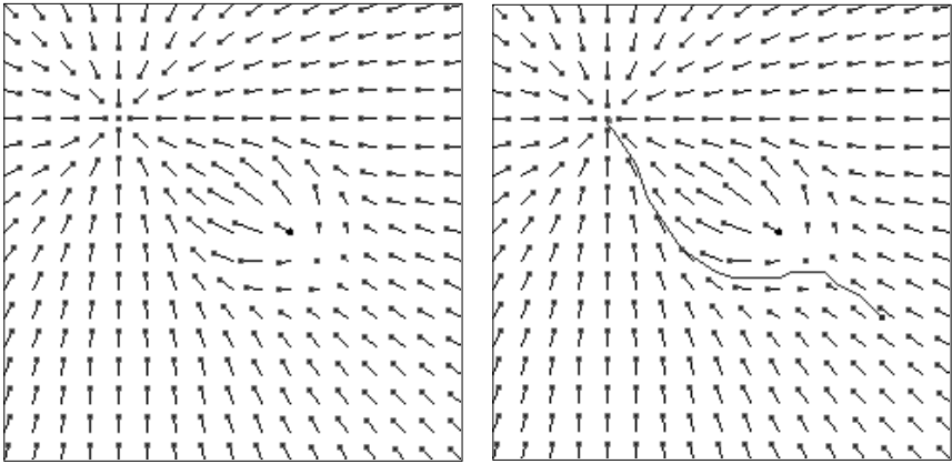
Fig. 4.3. (Left) Superposition of attractor and repellor vector field; (Right) Trajectory towards state vector S_A^v under by-passing state vector S_R^v .
