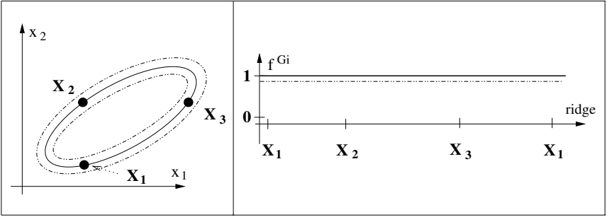
Fig. 3.8. (Left) Input space with three particular points from which a 2D ellipse is defined by PCA, small deviations from this ellipse are constrained by an inner and an outer ellipse; (Right) Result of function f^{Gi} along the ellipse, which is constant 1, accepted deviations are indicated by horizontal lines with offset \mp\zeta .
